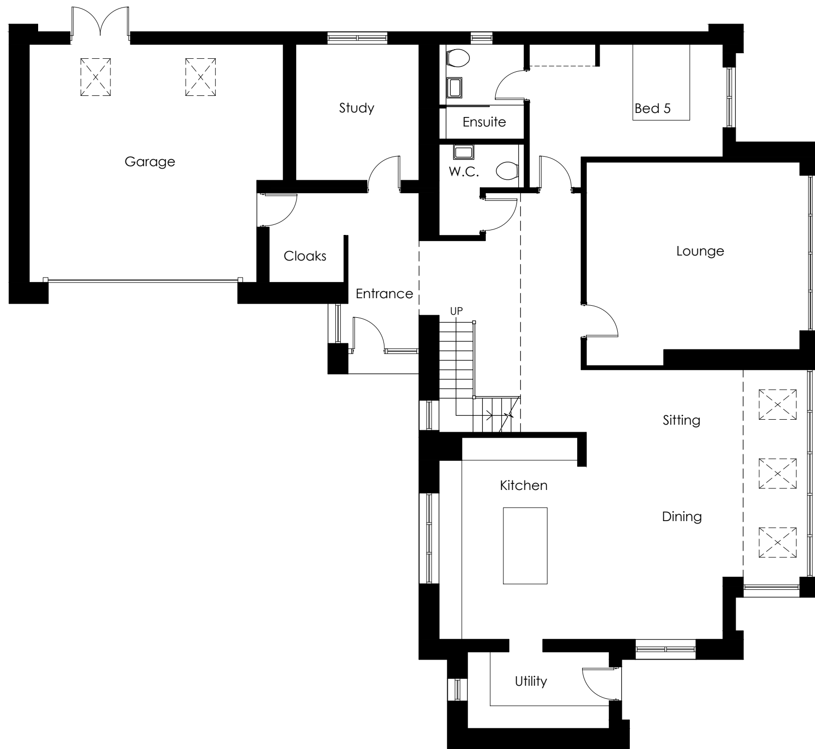
GROUND FLOOR
